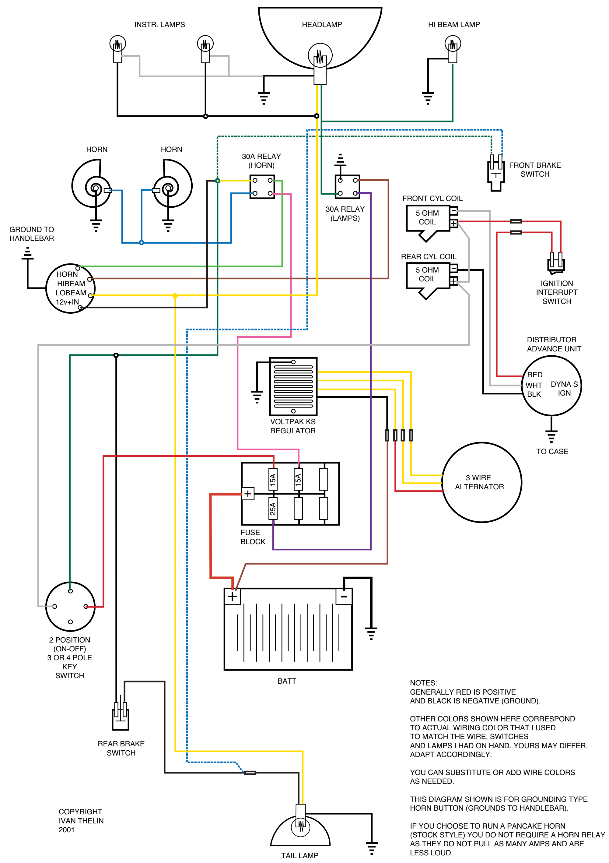
SIMPLIFIED WIRING DIAGRAM FOR DUCATI 750 GT BEVEL TWINS
